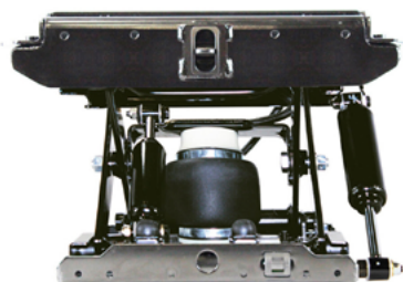
Double Damper View
