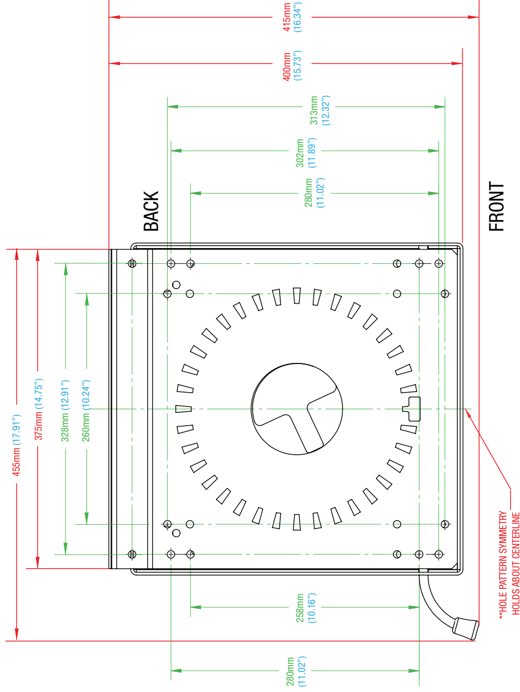
Bottom Mounting Pattern
