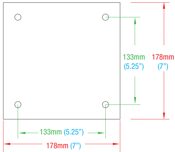
Bottom Mounting Pattern
