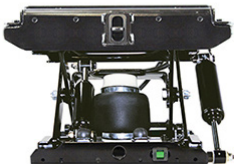
Double Damper
