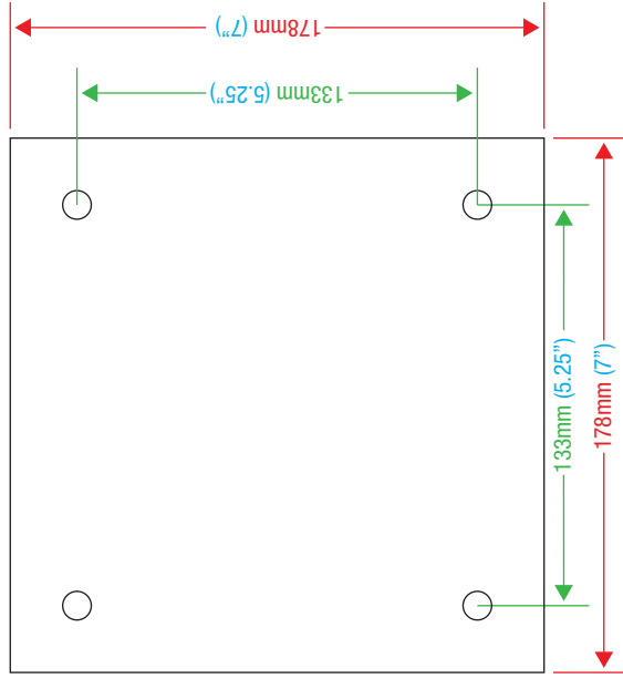
BOTTOM MOUNTING PATTERN
