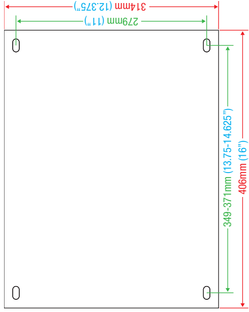
TOP MOUNTING PATTERN
