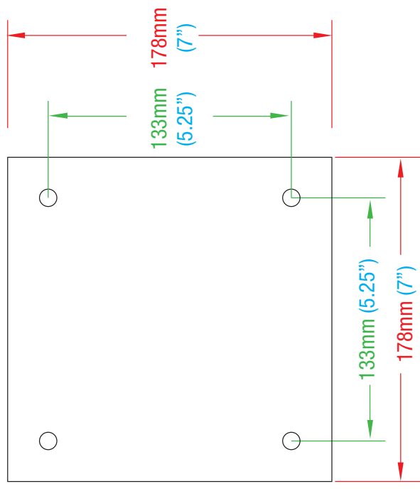
Bottom Mounting Pattern
