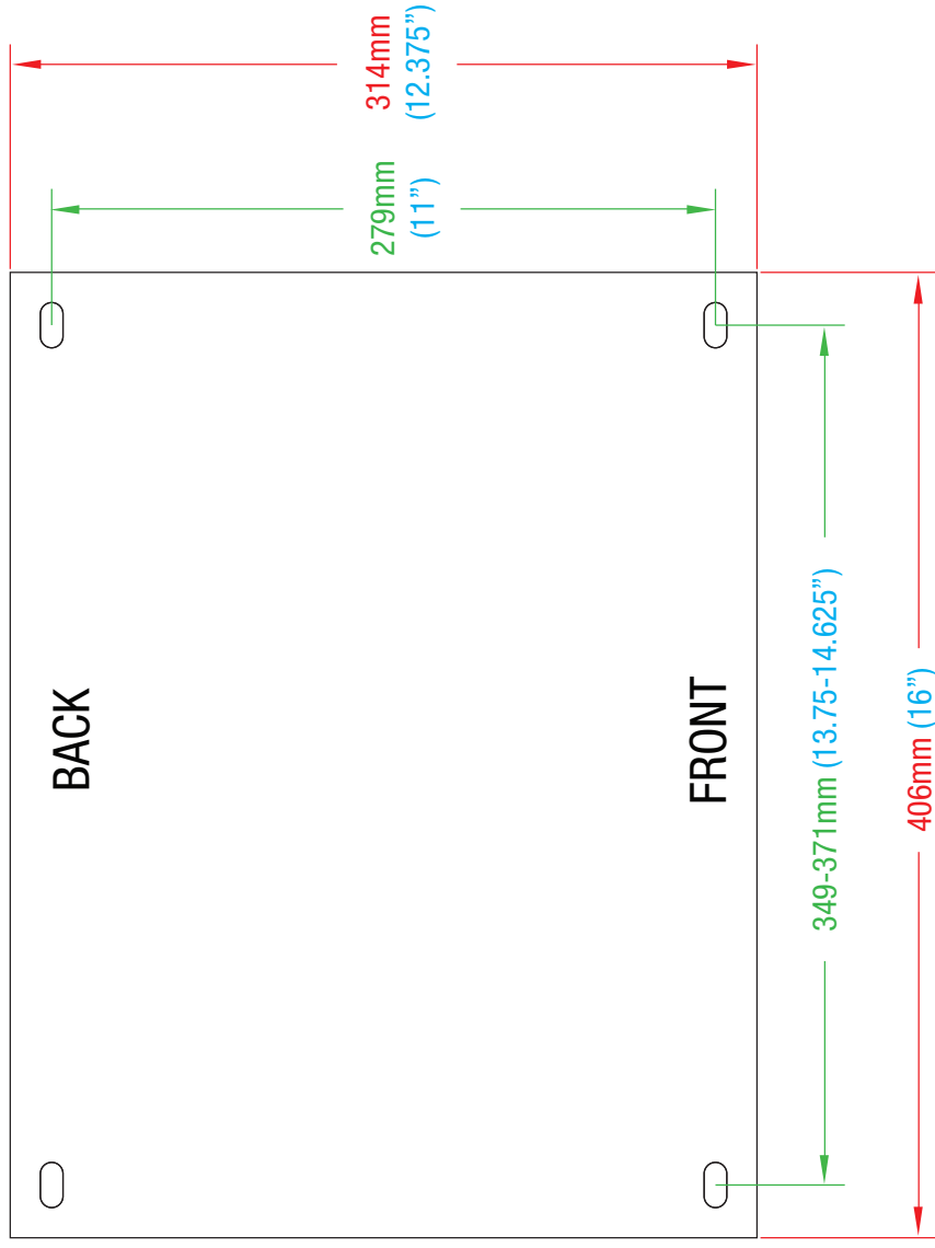
Top Mounting Pattern
